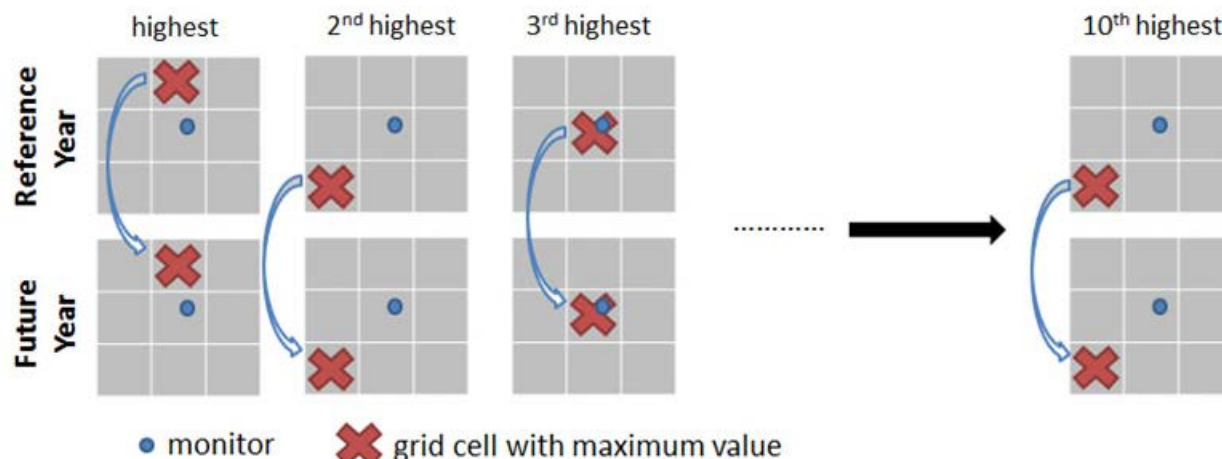
Figure B-3. Example showing how the location of the MDA8 ozone for the top ten days in the reference and future years are chosen.
