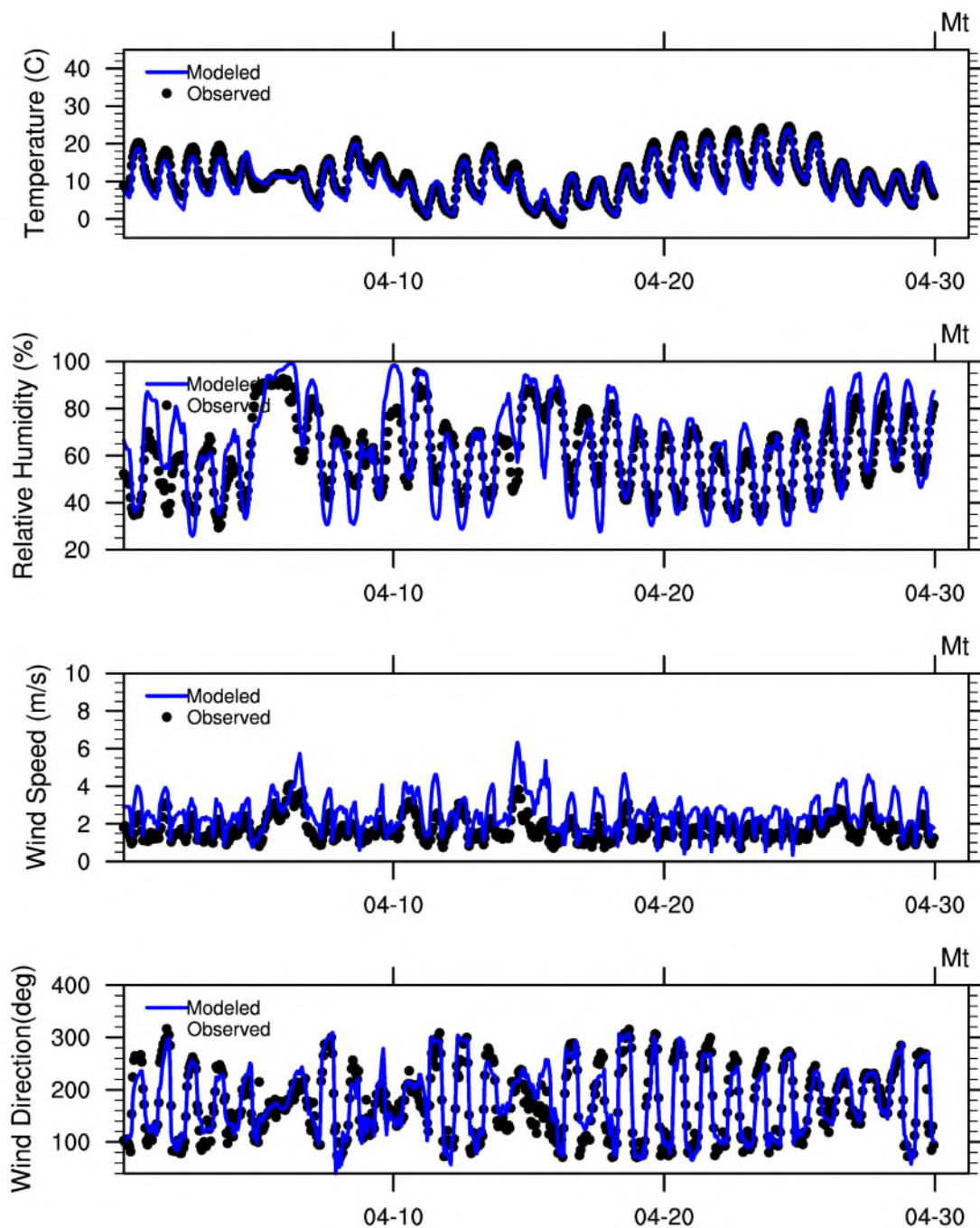
Figure S 2. Time series of average temperature, relative humidity, wind speed, and direction of all mountain sites in April 2018.
