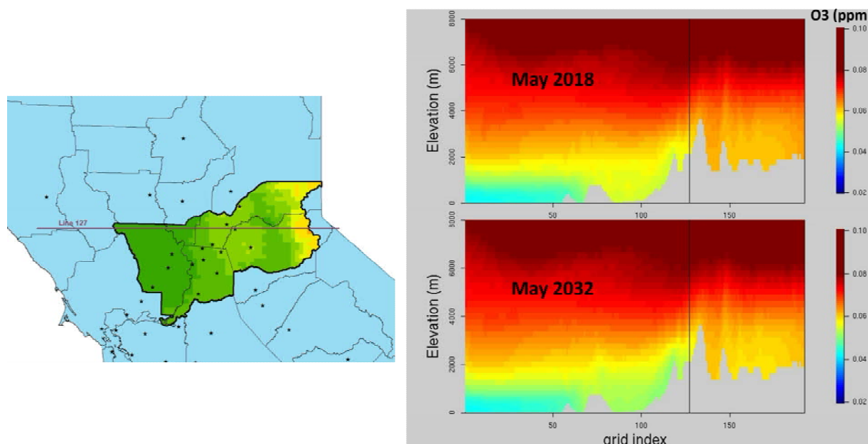
Figure S 61. Curtain plot of monthly averaged 8 hour O 3 concentrations in May 2018 and 2032 along row 127 of modeling domain.
