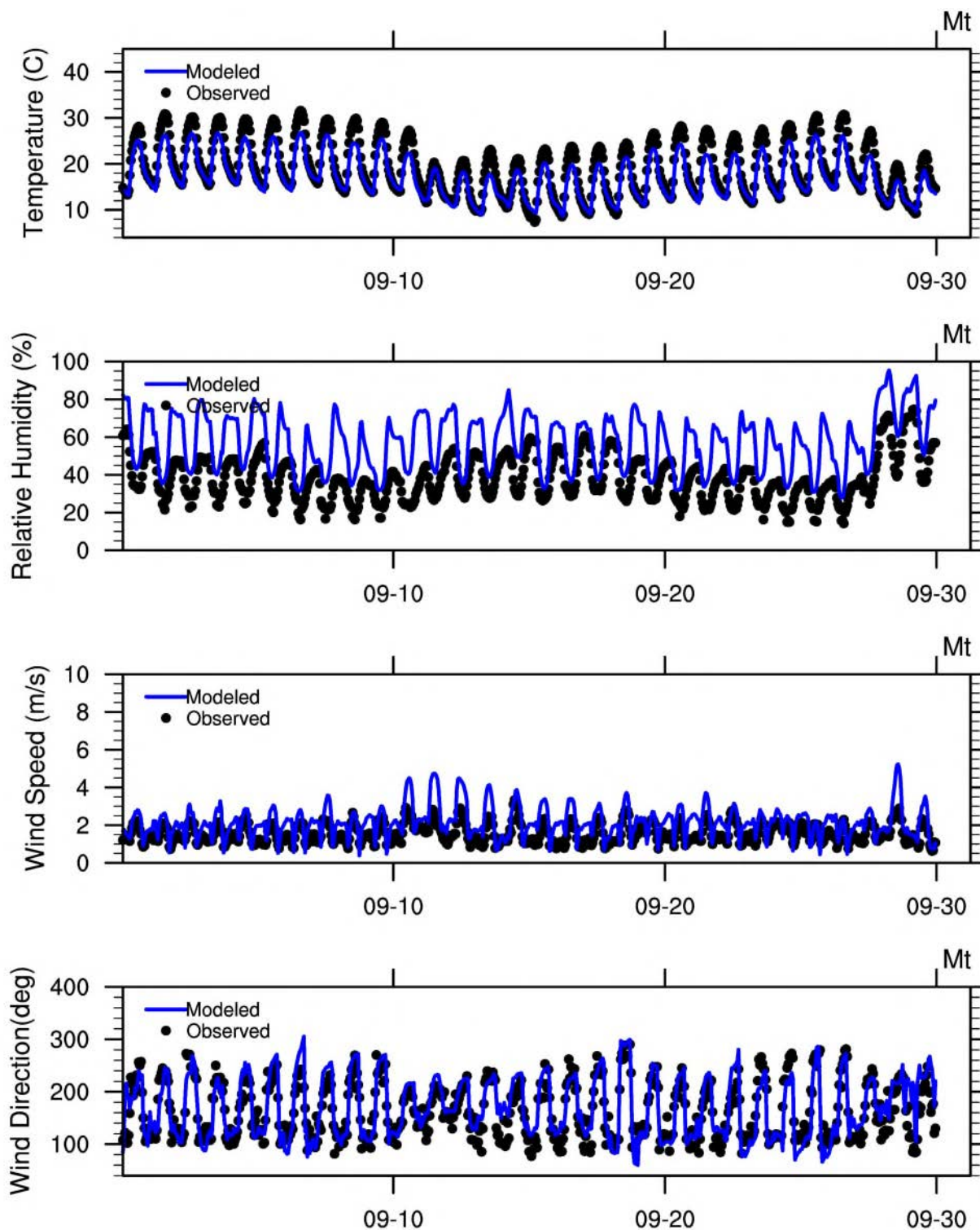
Figure S 12. Time series of average temperature, relative humidity, wind speed, and direction of all mountain sites in September 2018.
