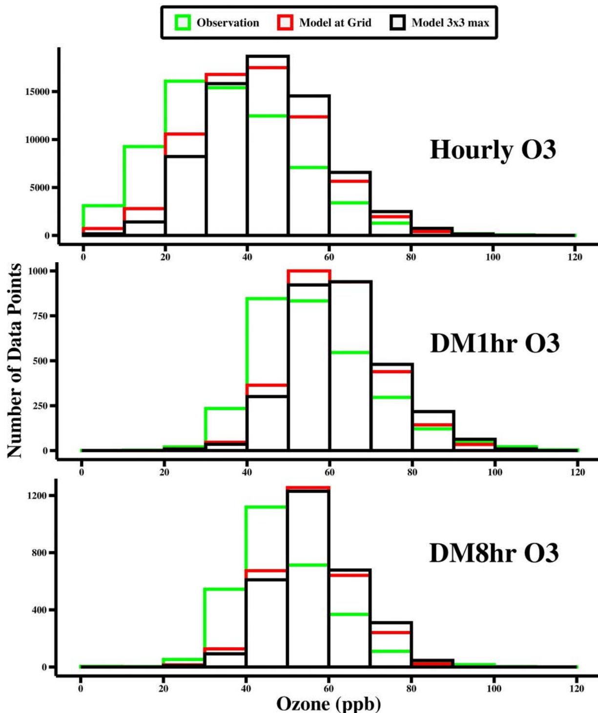
Figure S 16. Observed and modeled ozone frequency distribution for the ozone season in the SFNA (Fire days excluded in April – October 2018)
